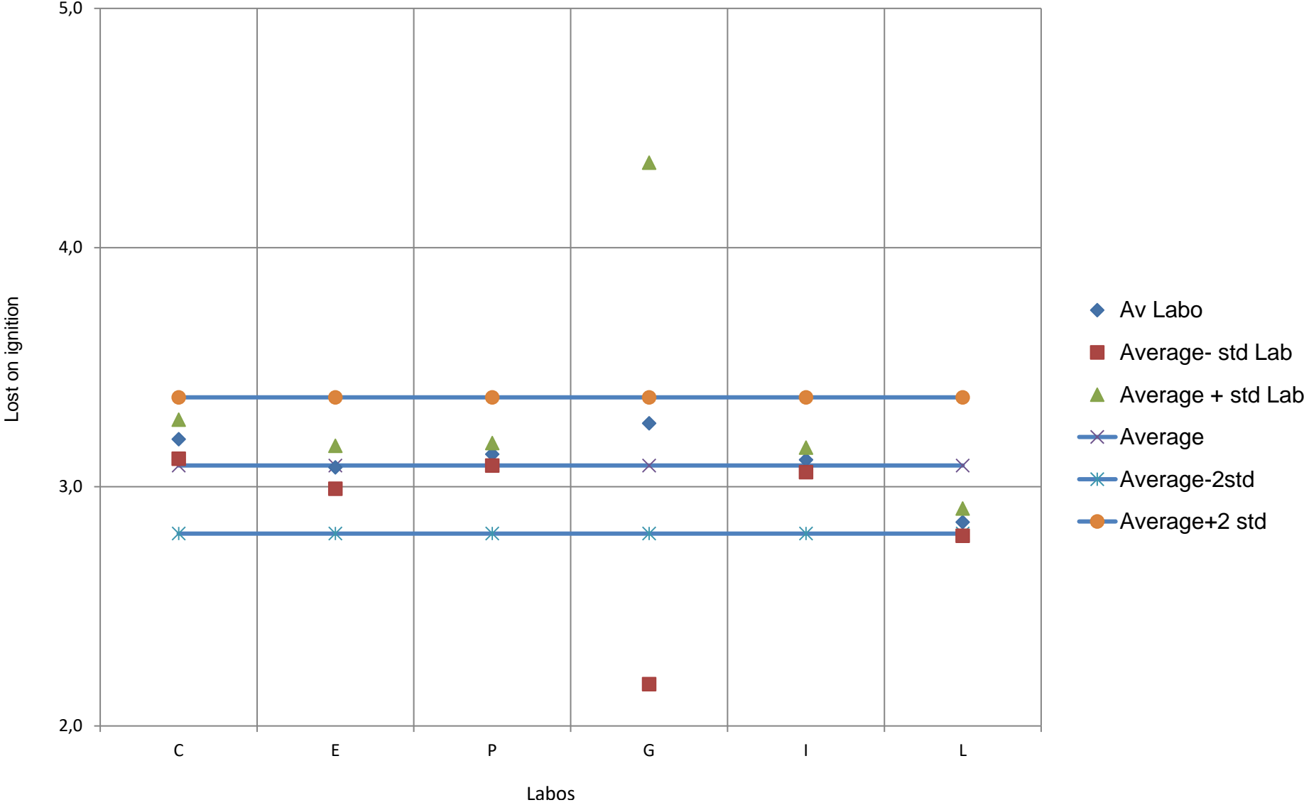
BE-CERT Round Robin Test Fly-Ash - 2015-2017 - Lost on ignition
