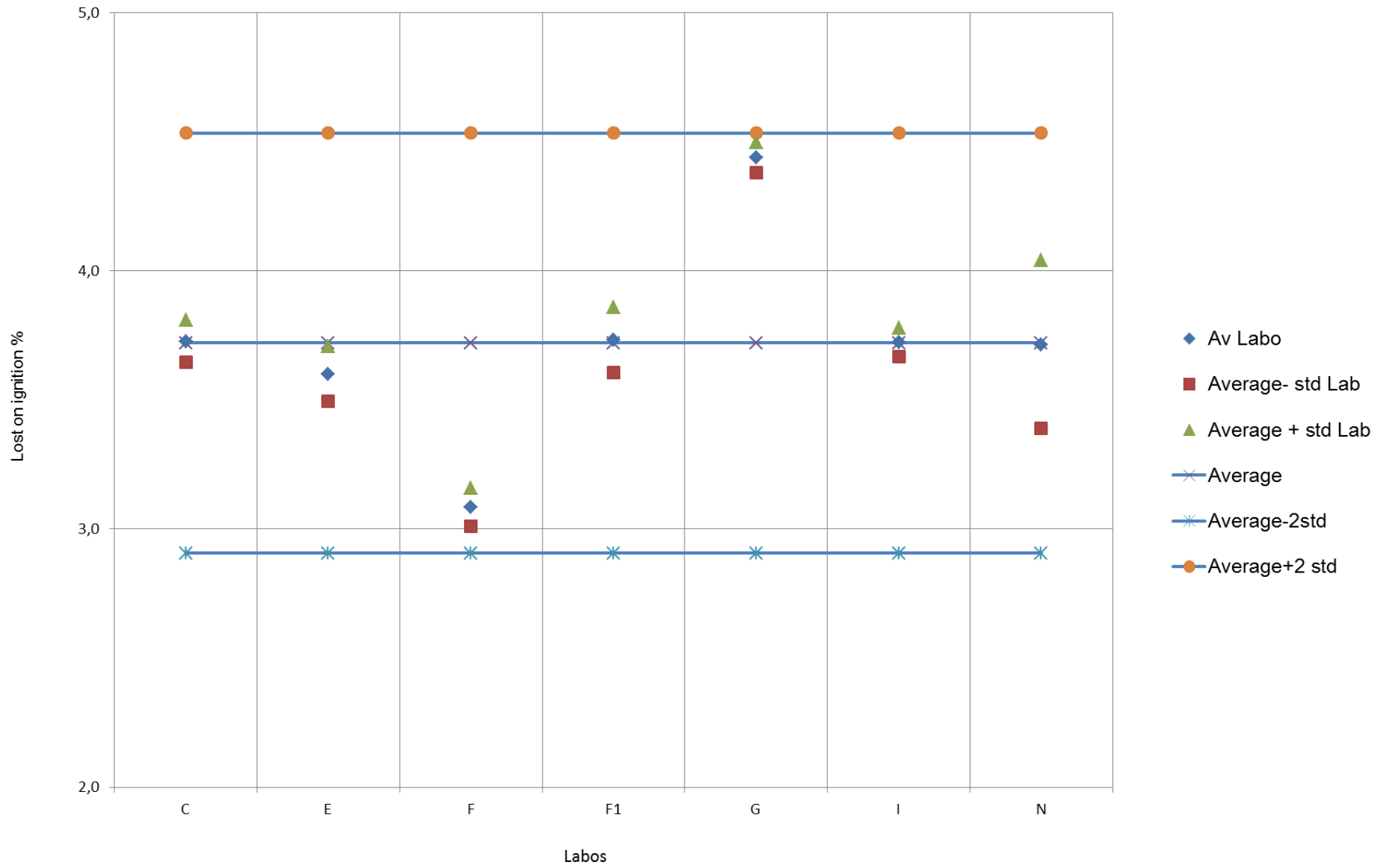
BE-CERT Round Robin Test Fly-Ash - 2013-2015 - Lost on ignition
